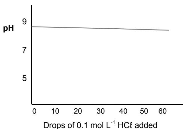
Graph 1. The change in pH when adding dilute HCl to an aqueous mixture of \text{NH}_3/\text{NH}_4\text{Cl}
